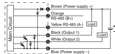
EFP02-□-02 NPN Output, RS-485 Modbus
