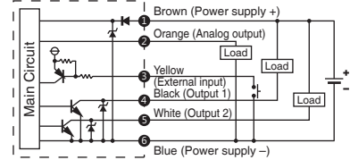
EFP02-□-011 NPN Output / Analog Current Output / External Input
