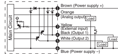
EFP02-□-031 PNP Output / Analog Current Output / External Input
