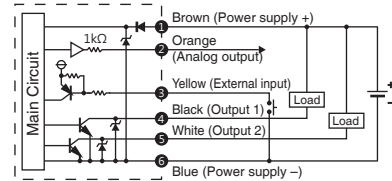
EFP02-□-010 NPN Output / Analog Voltage Output / External Input
