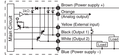
EFP02-□-030 PNP Output / Analog Voltage Output / External Input
