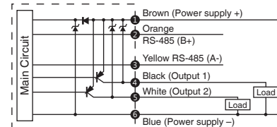
EFP02-□-04 PNP Output, RS-485 Modbus
