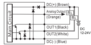
EP43 □ -02- □ 2 NPN+Copy Function
